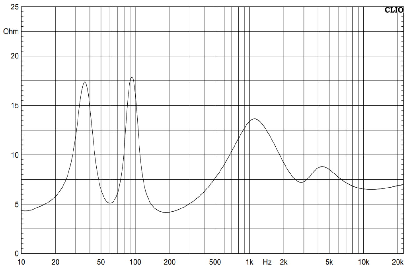
IMPEDANCE CURVE
