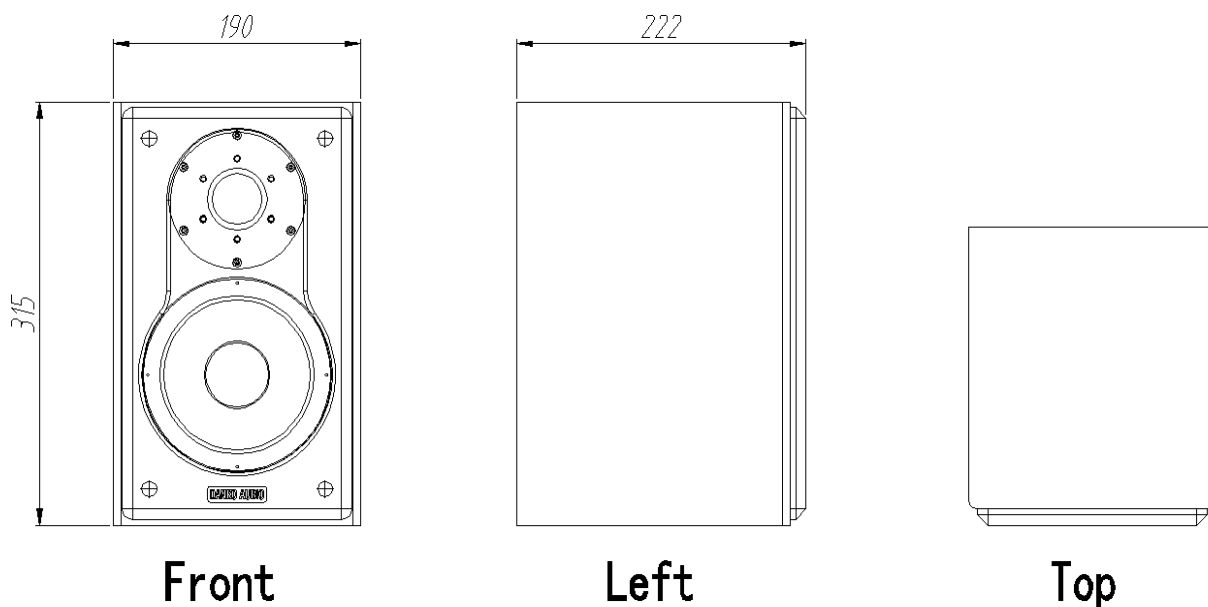
DIMENSIONS mm(in.)
