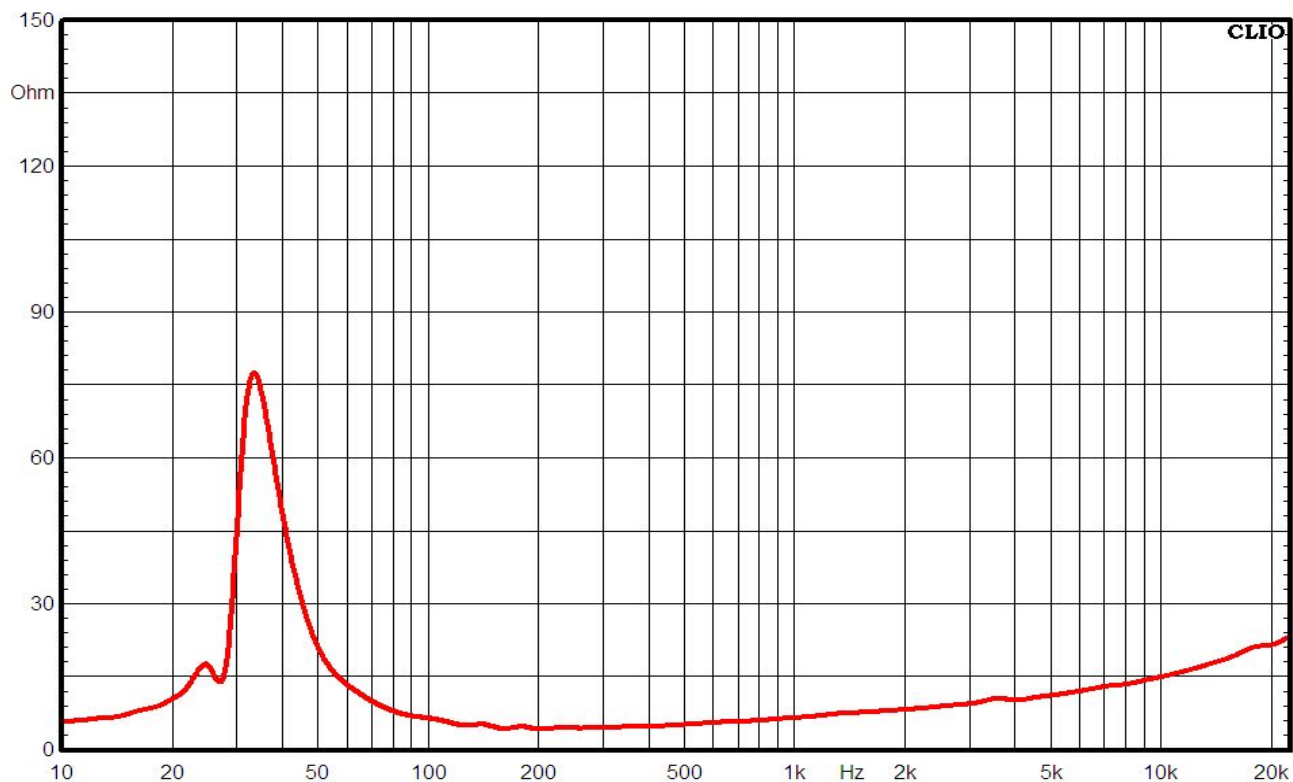
IMPEDANCE CURVE
