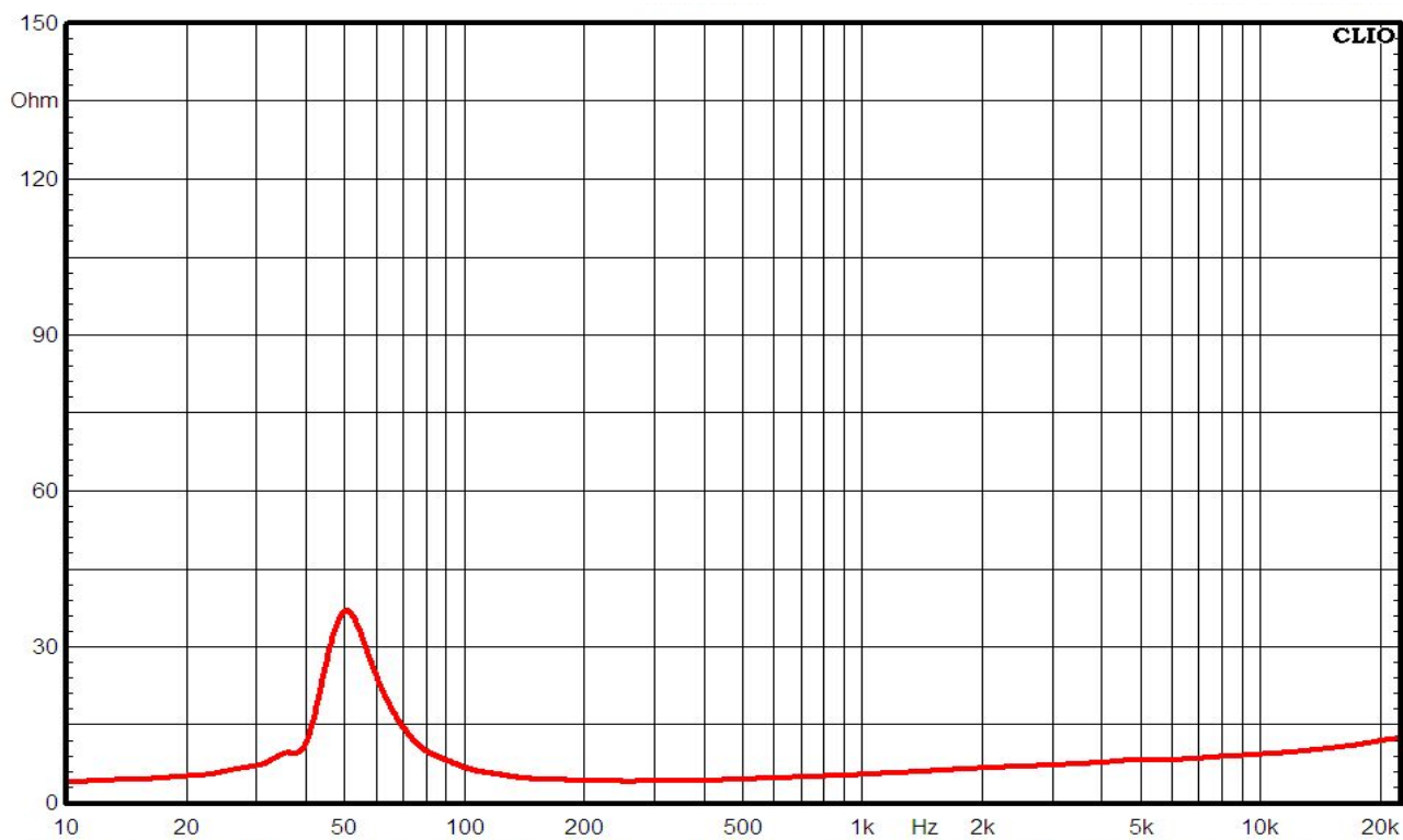
IMPEDANCE CURVE
