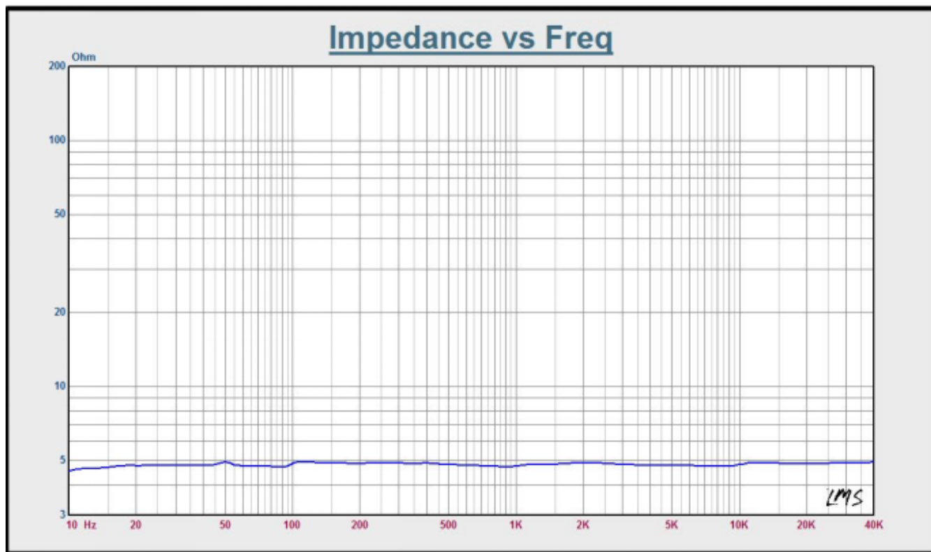
IMPEDANCE CURVE
