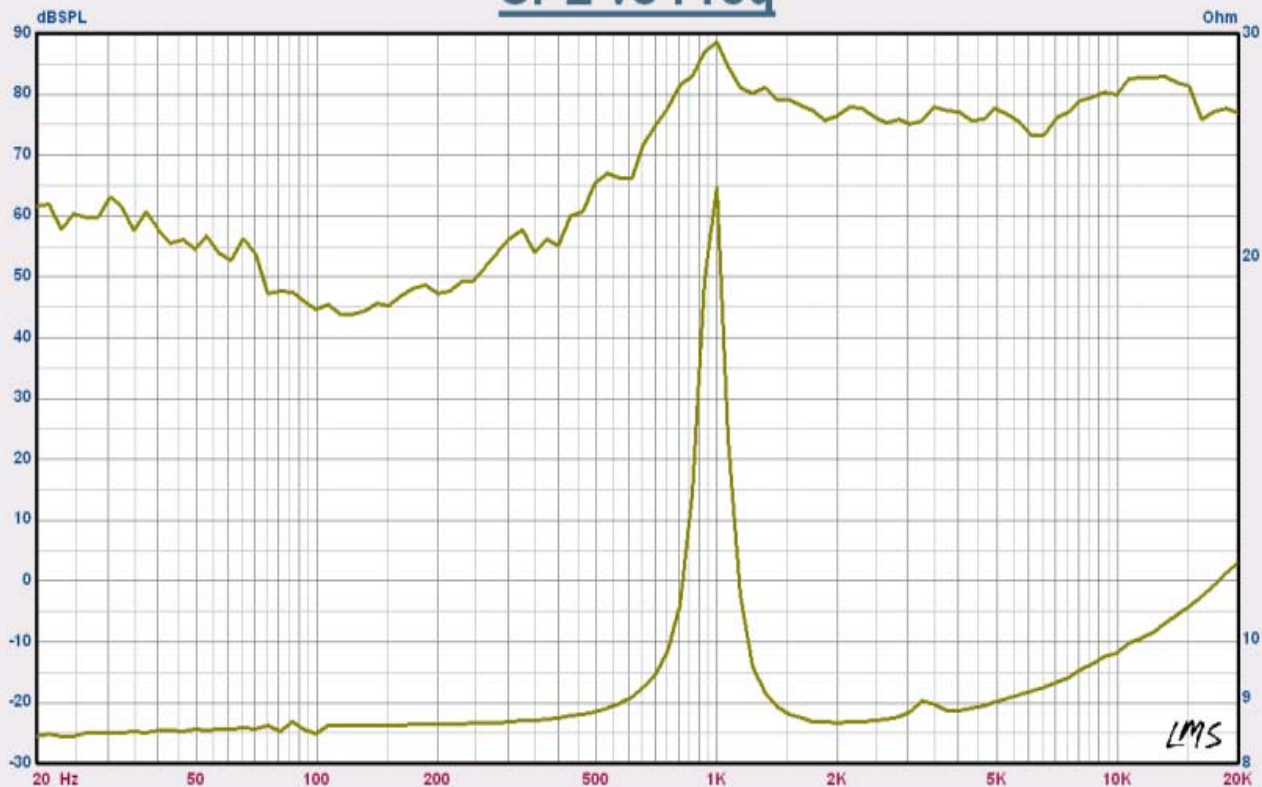
SPL vs Freq
