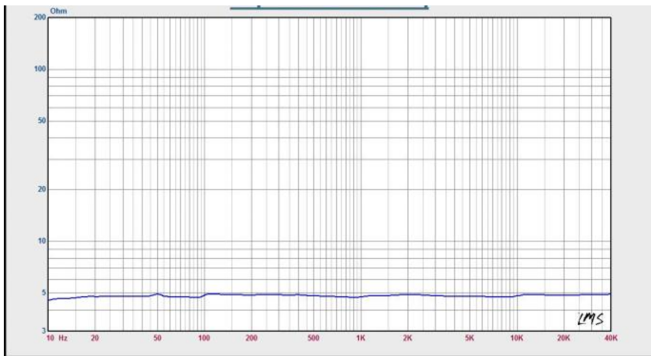
IMPEDANCE CURVE
