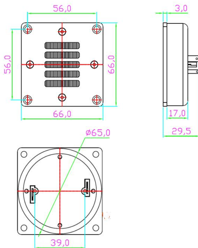
DIMENSIONS mm(in.)
