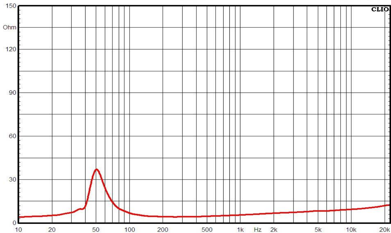
IMPEDANCE CURVE
