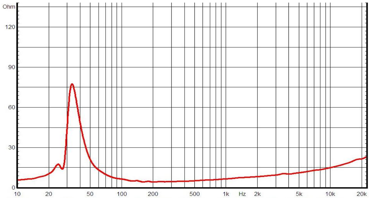
IMPEDANCE CURVE
