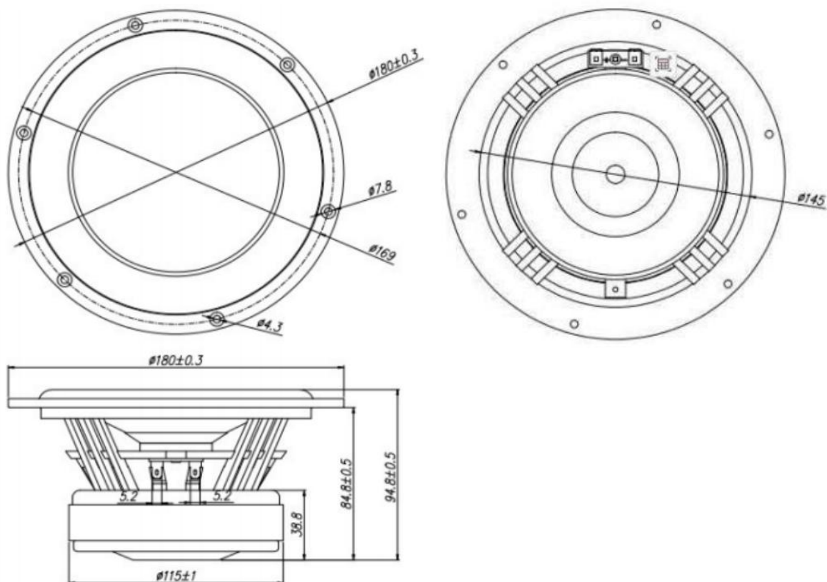
DIMENSIONS mm(in.)
