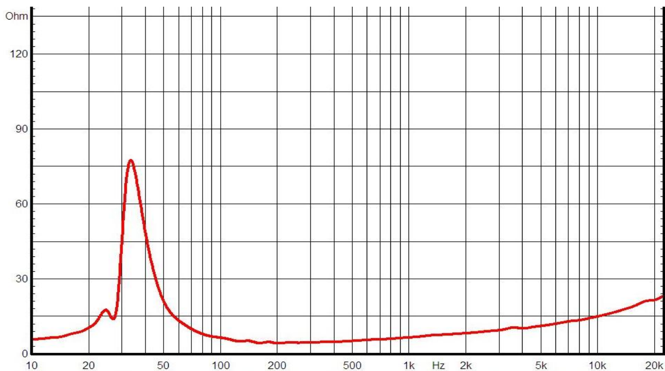
IMPEDANCE CURVE
